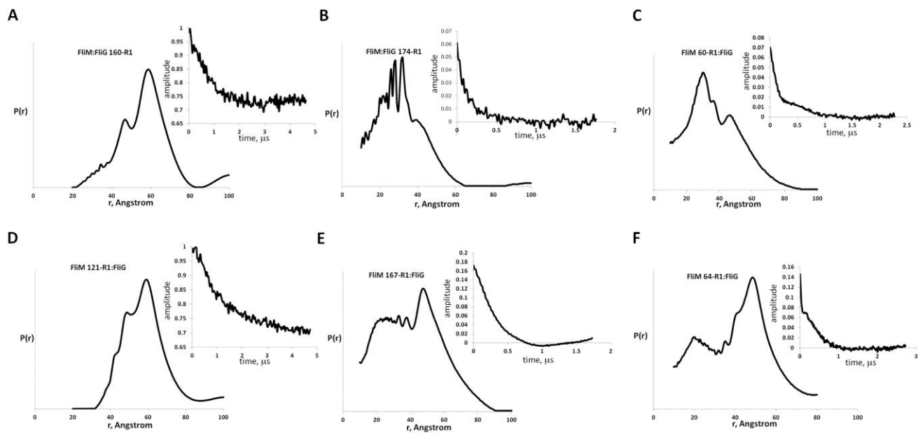
Figure S3. Distance distribution and time domain signal for spin label at (A) FliG 160-R1:FliM, (B) FliG 174-R1:FliM, (C) FliM 60-R1:FliG, (D) FliM 121-R1:FliG, (E) FliM 167-R1:FliG and (F) FliM64-R1:FliG. For (A) and (D), the measurement was performed in D_2O .
