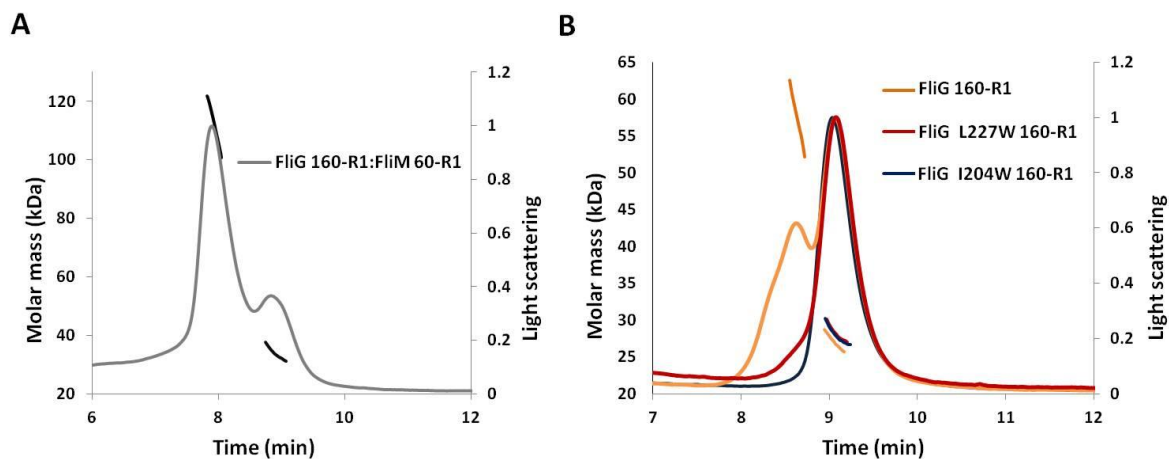
Figure S2. Multi-angle light scattering data on (A) FliG 160-R1:FliM 60-R1 showing formation of heterotetrameric complex (112 kDa) and excess FliM (33.7 kDa) under the conditions of the PDS experiment. Measurement with unlabelled protein also showed tetramer formation (data not shown) (B) FliG 160-R1 alone is a mixture of monomer (28.1 kDa) and dimer (57.3 kDa) whereas FliG L227W 160-R1 and FliG I204W 160-R1 behave as monomers (27.8 kDa and 27.1 kDa respectively). Unlabelled FliG also exists as a monomer in equilibrium with higher molecular weight species (data not shown).
