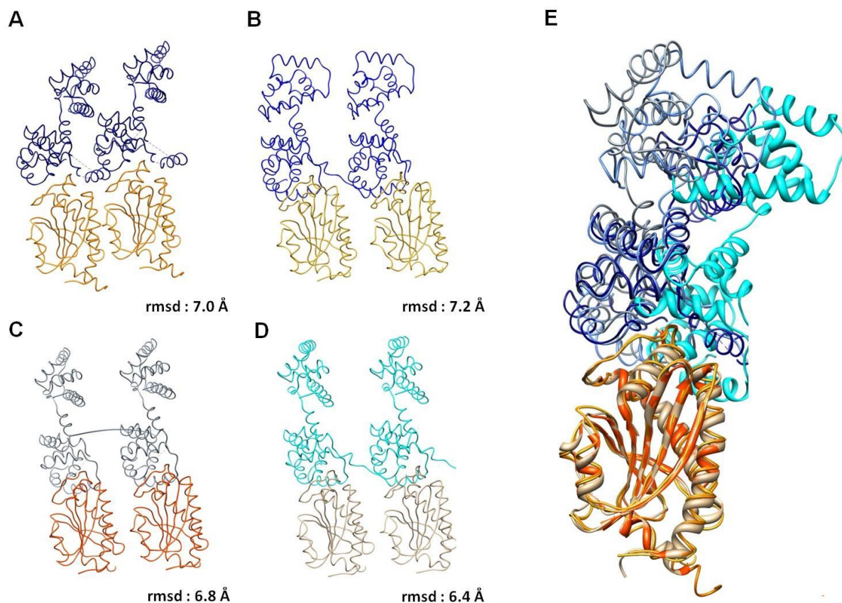
Figure S4. Different versions of model III used for fitting (A-D) with the corresponding rmsd with respect to the fit is indicated below. (E) Superposition of the FliM:FliG heterodimers from each version of model III tested (A-D).
