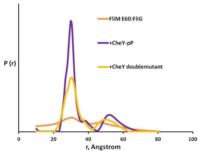
Figure S7. Changes in FliM spin distributions with activated CheY variants. Distance distributions for spin labels at FliM 60-R1:FliG (orange), with double mutant CheY(yellow), and with CheY-pP (purple).
