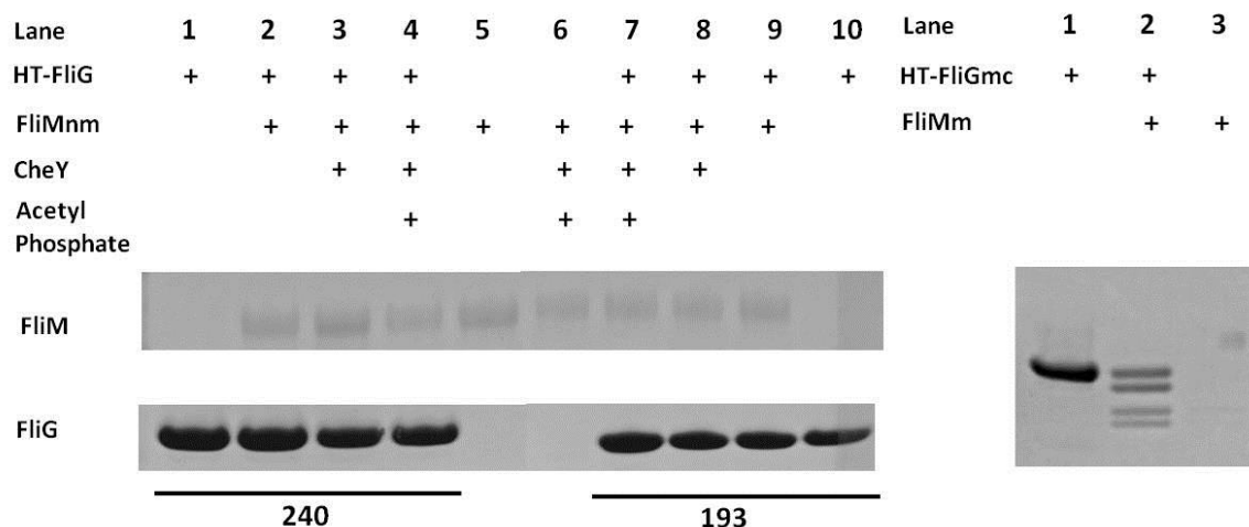
Figure S1. Interaction between FliM and FliG C . Left: Pull-down assay of FliM NM with FliG C 240 (residues 240-335) (lanes 1-4) and FliG C 193 (residues 193-335) (lanes 7-10) in presence of CheY or CheY-P where indicated. Controls of FliM NM without tag (lane 5) in presence of CheY-P (lane 6) show some non specific binding to the affinity beads. No apparent binding is observed between FliM NM and FliG C (240 in lane 2 and 193 in lane 9) nor was it observed in presence of CheY (240 in lane 3 and 193 in lane 8) or CheY-P (240 in lane 4 and 193 in lane 7). Right: Positive control experiment showing the interaction between His 6 -FliG MC (HT-FliG MC ) and FliM M (lane 2) performed under the same conditions as the samples on the left. Lanes 1 and 3 shows HT-FliG MC and FliM M respectively.
