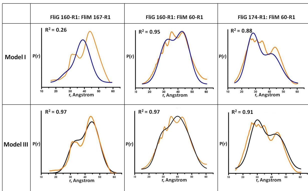
Figure S5. Qualitative analysis of distance distribution data using the antiparallel crystal structure (model I) for the fitting (top). Eqn 2 was used for fitting the anti-parallel arrangement of the FliM:FliG complex. Comparison of R^2 values and the envelope from the fitted Gaussian with the parallel model III (bottom) for each distribution indicates that model III act as a better model for the available data. In orange is the experimental distance distribution, blue curve is the sum of fitted Gaussian for model I and black curve is for model III.
