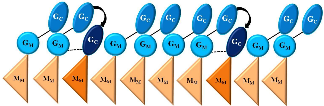
Figure S8. Possible arrangements of FliM and FliG based on the results from this study and the stoichiometry mismatch among the different rotor proteins. 26 copies of FliG interact with 26 copies of FliM (tan) through the middle domain. Gaps are created at the remaining 8 copies of FliM (dark orange) where no FliG M is present for binding. These 8 copies are likely randomly distributed in the C-ring. The C-terminal domains of a neighboring FliG (dark blue) may swing down and directly interact with FliM M through the conserved hydrophobic patch. This interaction between FliM and FliG C may only be observed in intact rotors.
