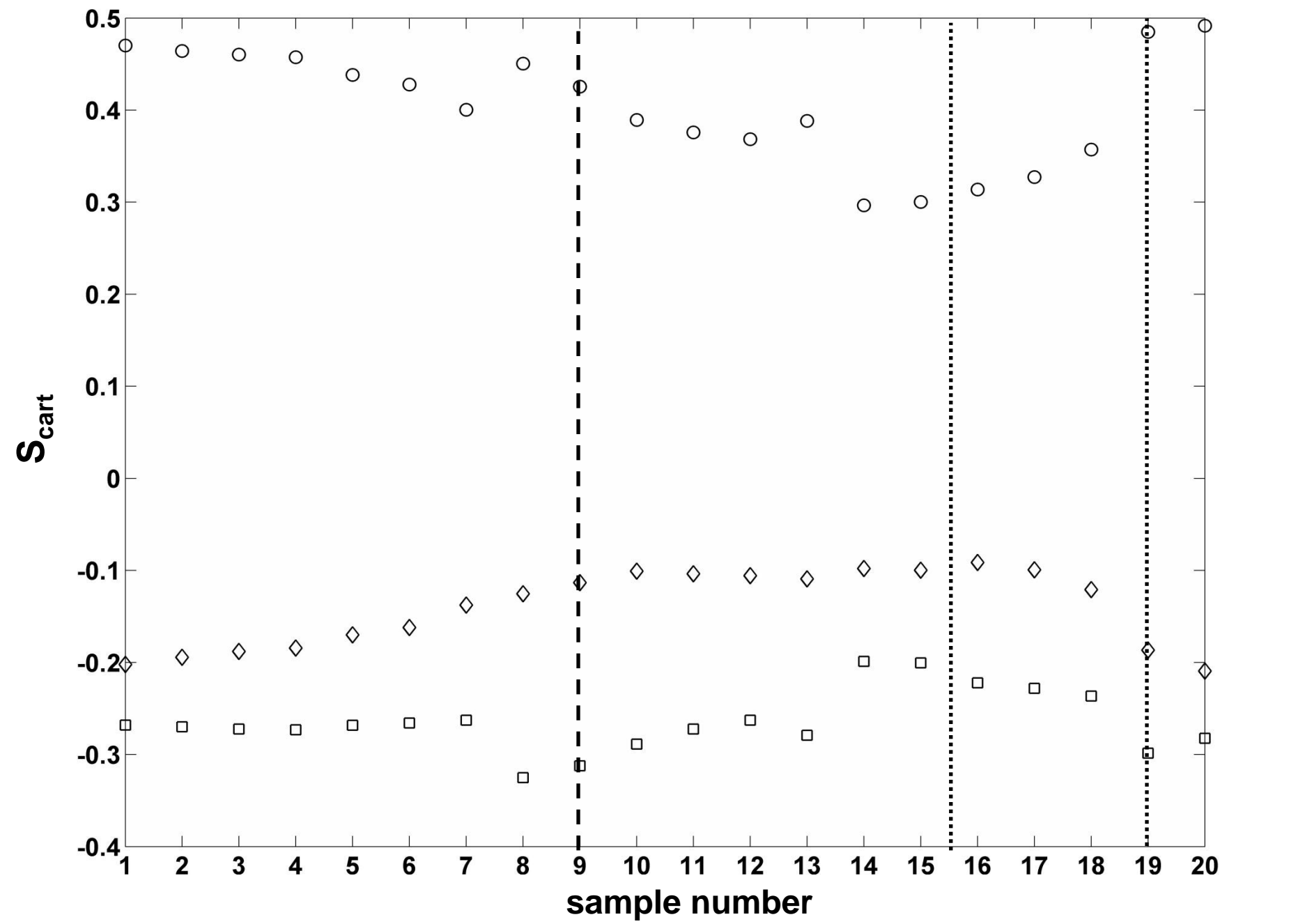
Supplementary Figure 16 SPMHEAD: S_{xx} (circles) S_{yy} (squares) S_{zz} (diamonds)
