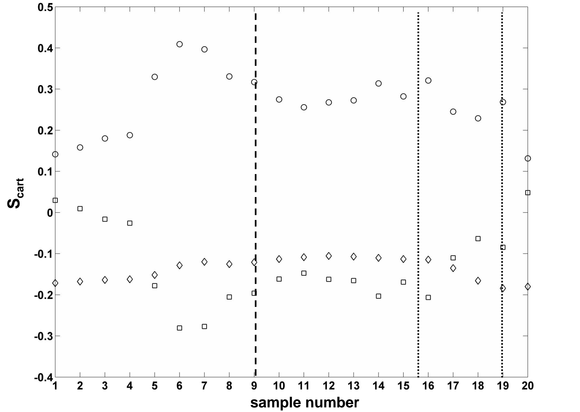
Supplementary Figure 15 DPPTC: S_{xx} (circles) S_{yy} (squares) S_{zz} (diamonds)
