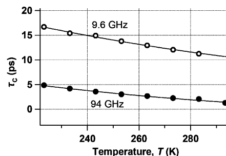
Figure 6. Characteristic electron correlation time \tau_c calculated by eq 6 using the observed T_1 and T_2 data for a 0.04 MPM lithium–ammonia solution at various temperatures. The solid lines are guides to the eyes only.
