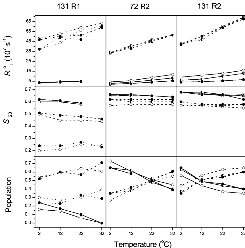
Figure 7. The best fit parameters of R_{\perp}^o , S_{20} , and the relative populations vs temperature from analysis of spectra recorded in water solution ( \circ ), in 15 w/v % Ficoll solution ( \bullet ), and in 25 w/v % Ficoll solution ( \bullet ); the immobile component (solid line), the intermediate component (dashed line), the mobile component (dotted line).
