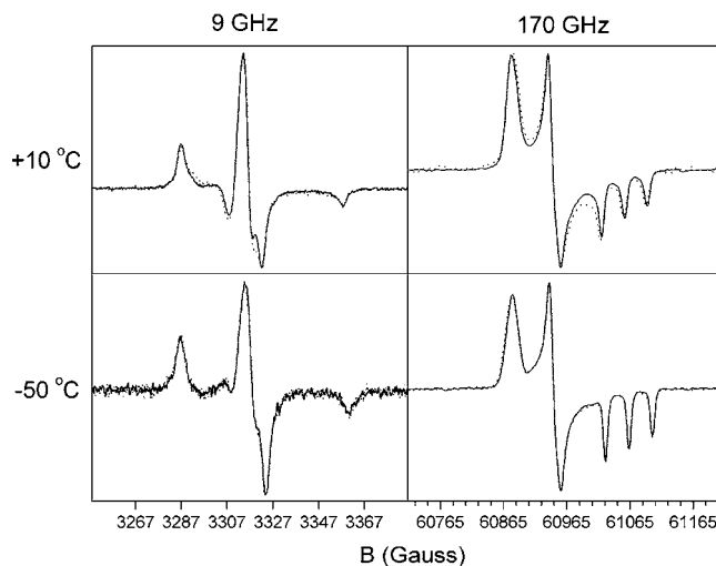
Figure 11. Comparison of spectra of 72R1 (solid line) and 131R1 (dashed line) recorded in 65 w/w% sucrose solution at +10 and -50 ^{\circ}\text{C} .
