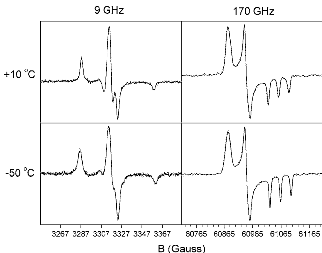
Figure 10. Comparison of spectra of 72R2 (solid line) and 131R2 (dashed line) recorded in 65 w/w% sucrose solution at +10 and -50 ^{\circ}\text{C} .
