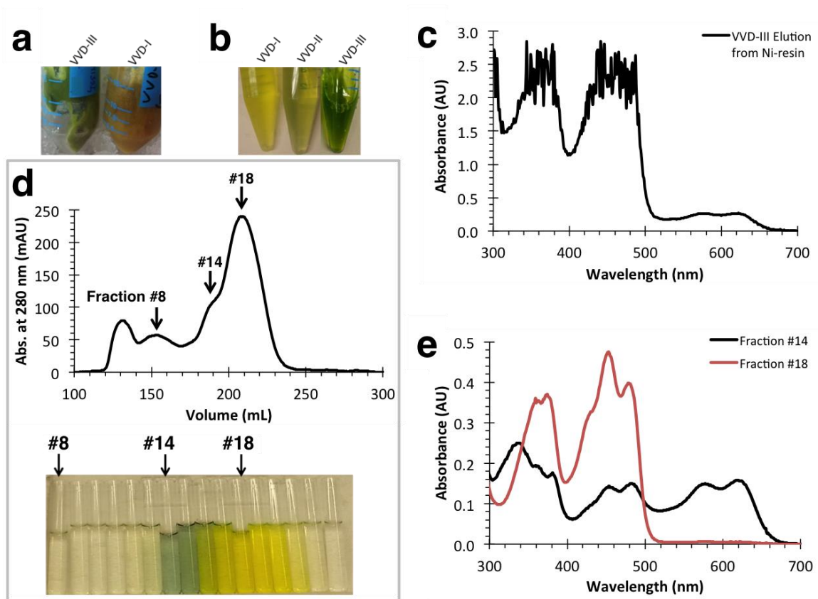
Supplemental Figure 1. VVD-III purifies in a reduced state. (a) The cell pellet of VVD-III (VVD \Delta 36 C108A:M135I:M165I) is green compared to VVD-I (wild type VVD \Delta 36 ) due to the accumulation of the neutral semiquinone radical. (b) Purified VVD-I is yellow, VVD-II (VVD \Delta 36 M135I:M165I) is pale green, while VVD-III is dark green. (c) Absorption spectrum of purified VVD-III, shown in (b), reveals a mixture of oxidized (450 nm) and neutral semiquinone (577 nm, 621 nm) states of FAD. (d) Size Exclusion Chromatography (SEC) profile of VVD-III shows that the different redox forms of VVD separate by size; fractions corresponding to the peaks are shown above. (e) Absorption spectra of fraction #14 (d), which elutes earlier than #18, contains a neutral semiquinone state of VVD-III, whereas #18 contains the oxidized form.
