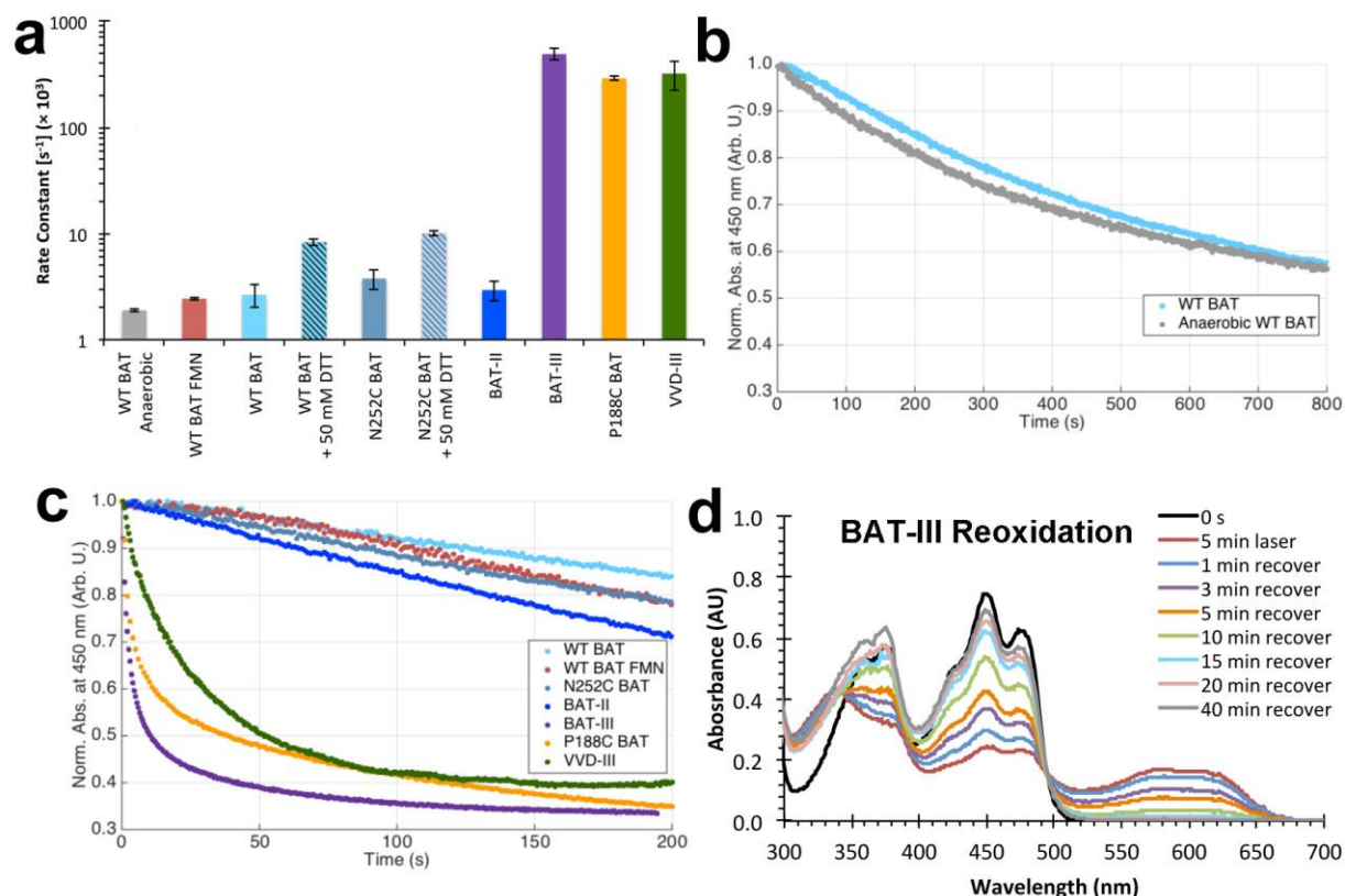
Supplementary Figure 6. Relative photoreduction yields of VVD-III and BAT-LOV*. (a) VVD-III reduces to the NSQ by orders of magnitude more rapidly than BAT-LOV* when exposed to 448-nm light. However, photoreduction yields of BAT-LOV* can be increased to rival those of VVD-III by either replacing the three flavin-proximal aromatic residues (BAT-III) with Phe or substituting the Pro residue that occupies the position which normally forms an adduct with a Cys residue (P188C). Addition of a Cys residue on I \beta ~13 Å from the flavin ring has only a small effect (N252C), as does addition of exogenous reductants. Reconstitution with FMN instead of FAD has an insignificant effect. (b) In the presence of air, there is a small lag phase for WT BAT-LOV* photoreduction that is not present under anaerobic conditions. (c) Time courses for photoreduction of VVD and BAT variants. (d) Recovery of photoreduced BAT-III to the oxidized state in aerobic solution.
