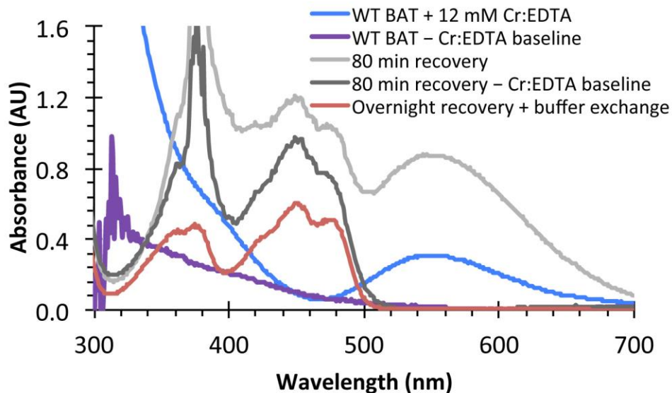
Supplementary Figure 7. Chemical reduction and recovery of BAT-LOV*. Treatment of BAT-LOV* with the low potential reductant Cr:EDTA generates a fully reduced flavin (blue line, broad absorption at 550 nm represents oxidation products of the Cr:EDTA reagent; purple line, with Cr:EDTA subtraction). Reoxidation after 80 min (shown with (dark grey) and without (light grey) Cr:EDTA subtraction) recovers the oxidized flavin, which is more evident after removal of the reductant by buffer exchange (red). A substantial amount of flavin remains bound to the protein after reoxidation.
