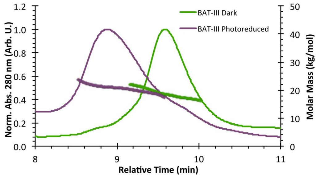
Supplementary Figure 8. Multi-angle light scattering of BAT-LOV* and BAT-III. (a) Molar mass measurements from MALS are shown across the SEC elution profiles for dark-adapted BAT-LOV*-FAD (black) and BAT-LOV* exposed to a 100 W broad-spectrum visible light source for 1.5 h prior to chromatography (blue). (b) MALS-SEC data of BAT-III in the dark-adapted and photoreduced state. The shift in BAT elution profile does not accompany a substantial change in molecular weight. Elution times are standardized to WT BAT-LOV*.
