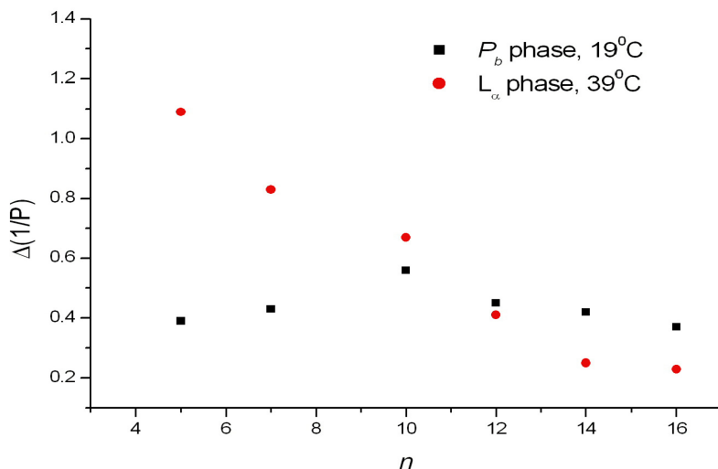
Figure 3. Relaxation enhancement from 10 mM of \text{Ni}(\text{ClO}_4)_2 introduced into the water phase of lipid DMPC dispersions as a function of n in the P_\beta (19°C) and L_\alpha (39°C) lipid phases. An almost flat accessibility profile in the gel might indicate similar average membrane immersion depth for the nitroxide moieties of all studied PC labels (from 16 ).
