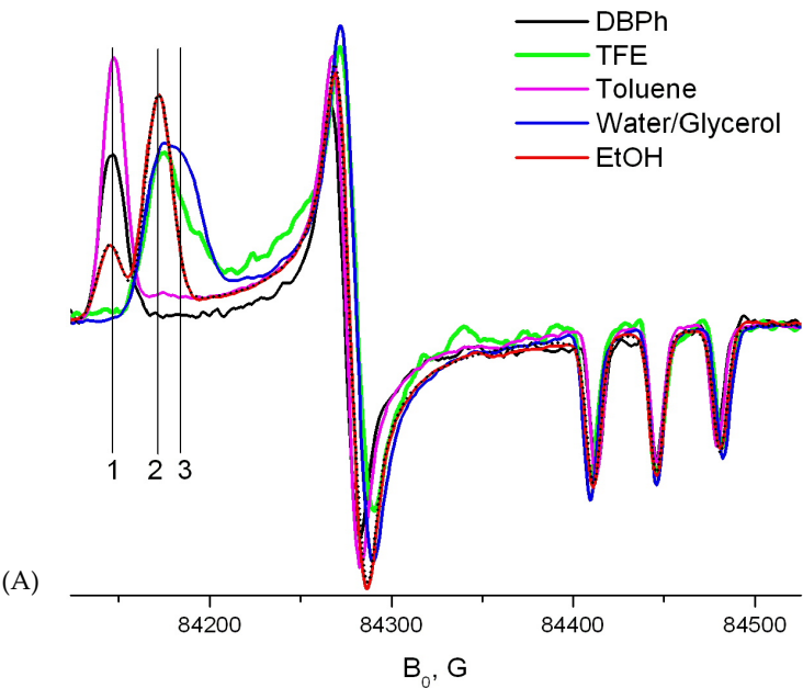
Tempone in different solvents, rigid limit
