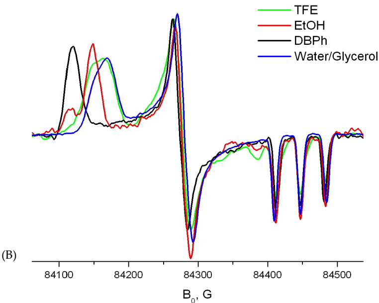
Tempol in different solvents, rigid limit
