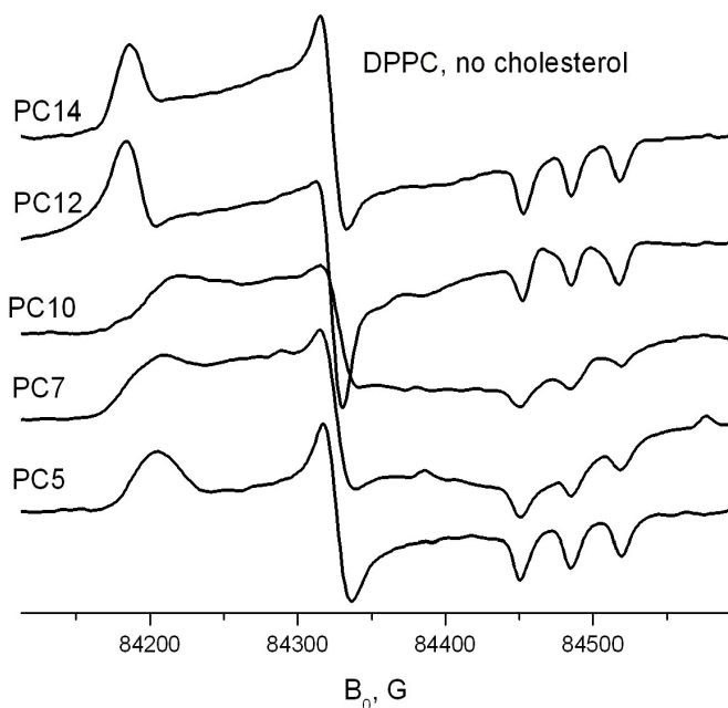
Figure 7. n -PC spin labels in DPPC with no cholesterol at 80–82K. The samples are gradually frozen in the flow of gaseous nitrogen (from 16 ).
