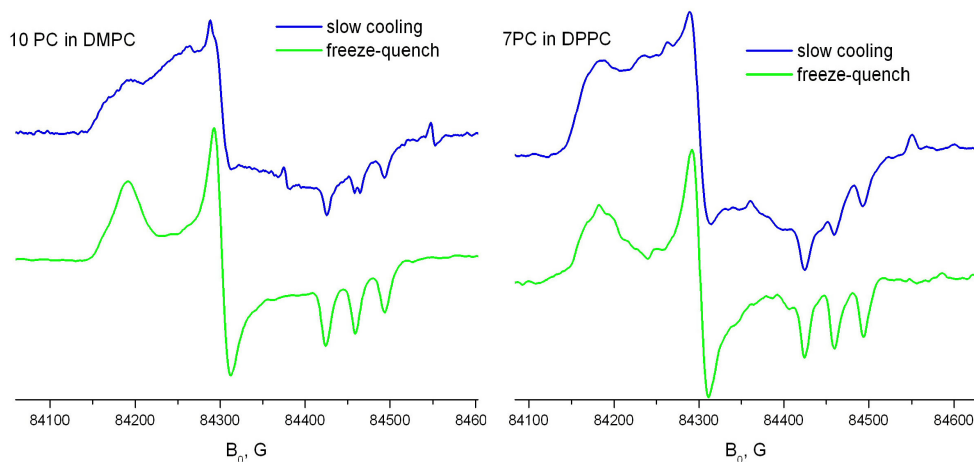
Figure 11. Obtaining better resolved spectra by quick freezing in liquid nitrogen (from 16 ).
