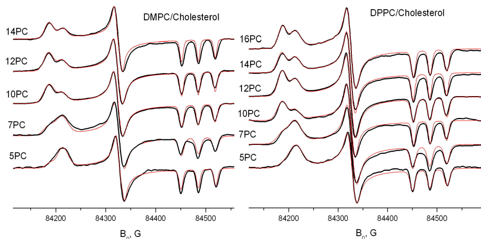
Figure 4. Rigid-limit 240 GHz ESR spectra of n -PC spin labels in DMPC and in DPPC containing 30% mol cholesterol. T=80 -82K. The samples are gradually frozen in the flow of gaseous nitrogen. Red lines show simulations of these spectra using two components with the g_{xx} = 2.009435 \pm 0.000005 and 2.008820 \pm 0.000005 for all spectra. g_{yy} and g_{zz} are taken 2.006100 and 2.00233 for both components (from 16 ).
